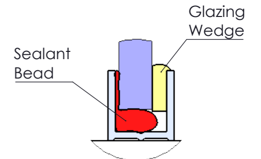
Glass Panel Silicone Detail
