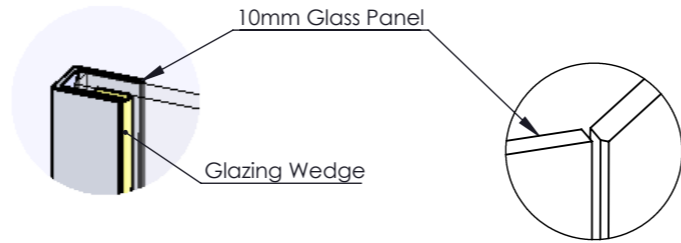
Glass To Wall Tolerance DETAIL A
