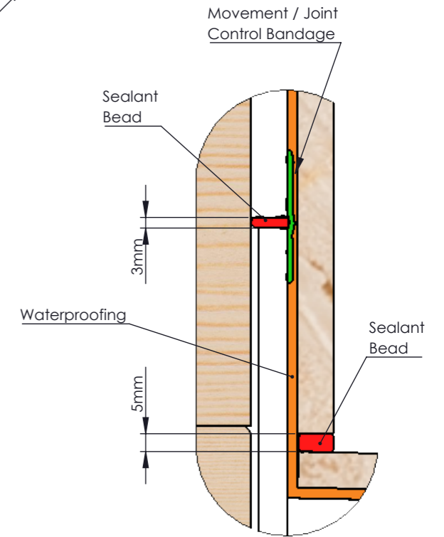
Wall Joint Detail DETAIL C
