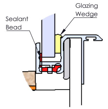
Glass Panel Silicone Detail DETAIL D
