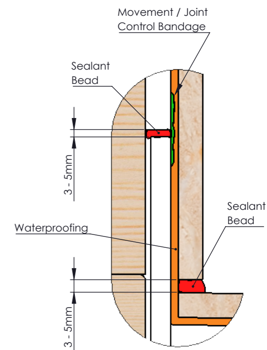
Wall Joint Detail DETAIL C
