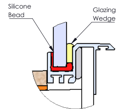
Glass Panel Silicone Detail
