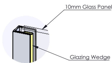
Glass To Wall Tolerance DETAIL A
