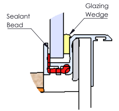
Glass Panel Silicone Detail DETAIL D
