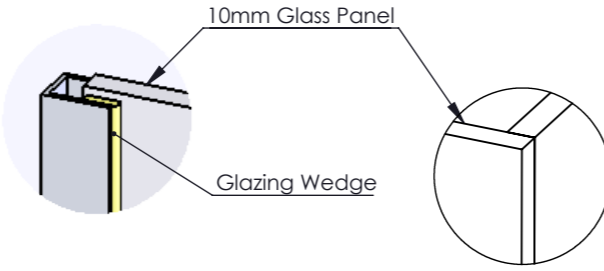
Glass To Wall Tolerance DETAIL A
