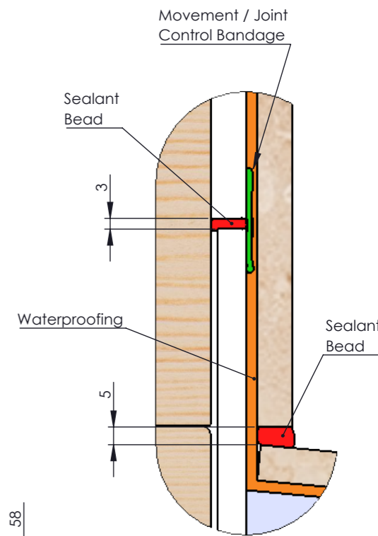
Wall Joint Detail DETAIL C
