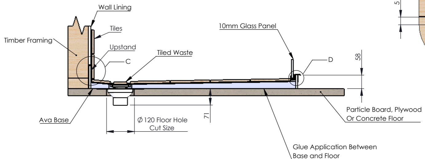
Wall Joint Detail DETAIL C
