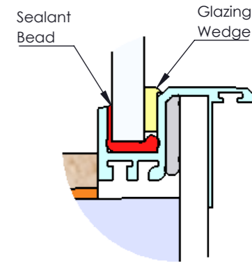
Glass Panel Silicone Detail DETAIL D
