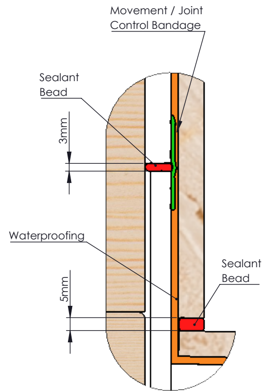
Wall Joint Detail DETAIL C
