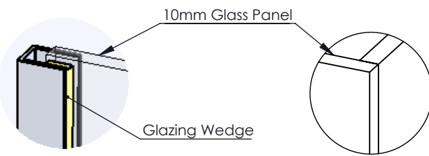
Corner Detail DETAIL B
