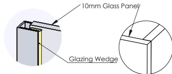
Glass To Wall Tolerance DETAIL A
