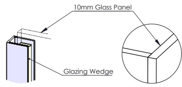
Glass To Wall Tolerance Rail Hidden DETAIL A
