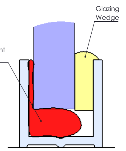
Glass Panel Silicone Detail DETAIL D
