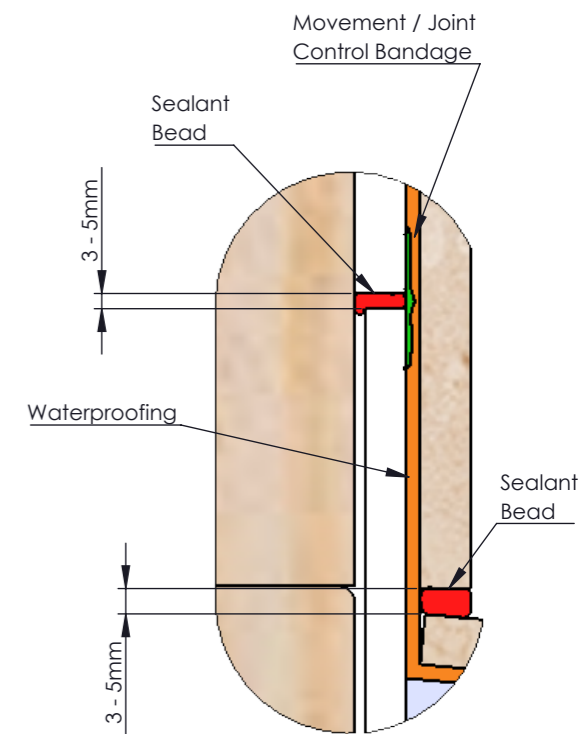
Wall Joint Detail DETAIL C
