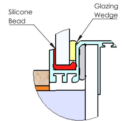
Glass Panel Silicone Detail
