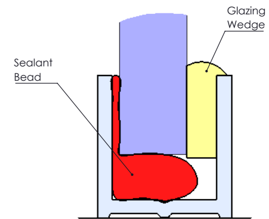
Glass Panel Silicone Detail DETAIL D
