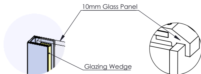
Glass To Wall Tolerance DETAIL A
