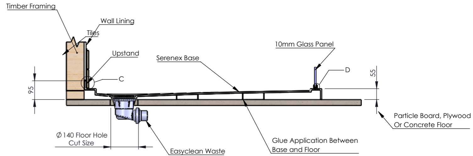
Corner Detail DETAIL B
