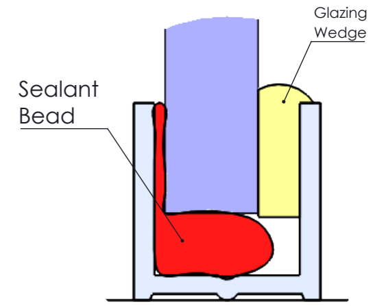
Glass Panel Silicone Detail DETAIL D
