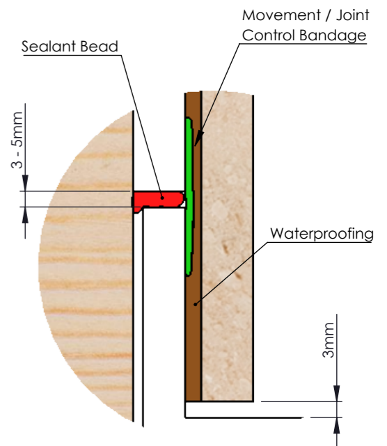
Wall Joint Detail DETAIL C
