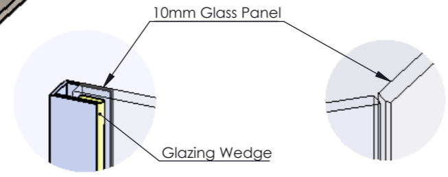
Glass To Wall Tolerance DETAIL A
